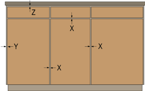
Figure 44 - Gaps, Flush Overlay Frameless
