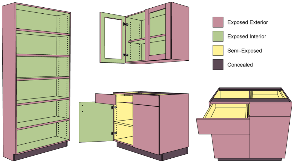
Figure 86 - Casework Surfaces
