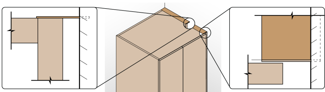
Figure 41 - Closure, Laminate
