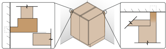
Figure 10 - Scribe Allowance
