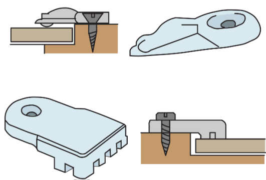
Figure 32 - Glass Clips
