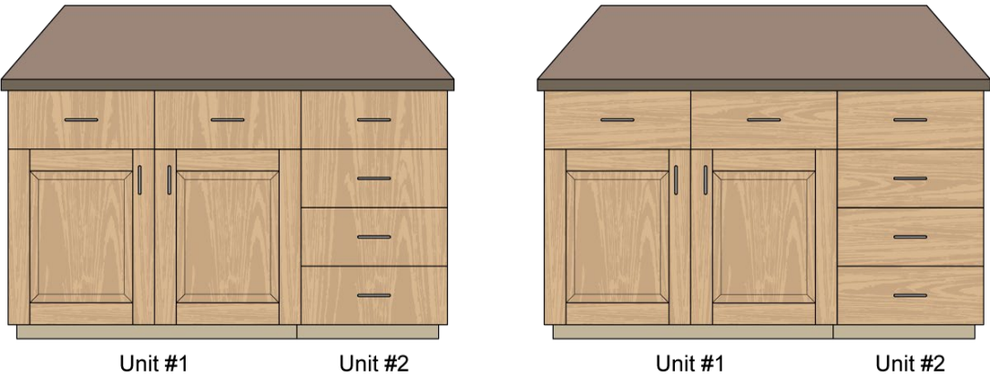
Figure 18 - Grain Layout, Stile and Rail 1
