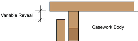
Figure 16 - Face Frame Construction Reveal
