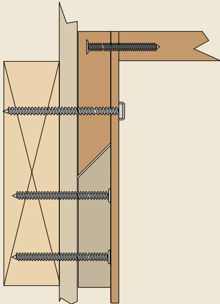
Locking Hanging Cleat
